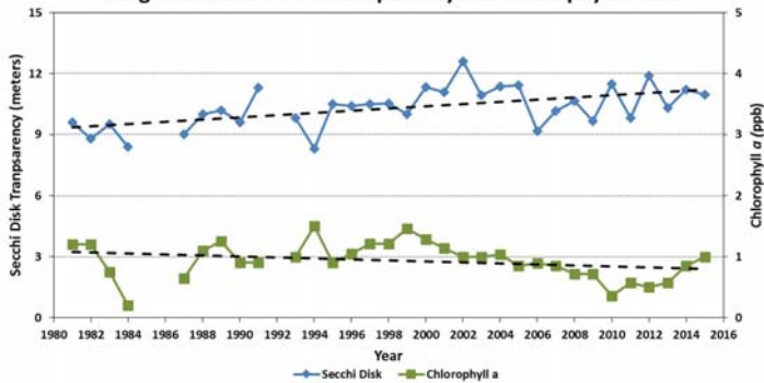
Figure 4. Merrymeeting Lake - Site 1 Broad Cove (1981-2015) Long-term Secchi Disk Transparency and Chlorophyll a Data
