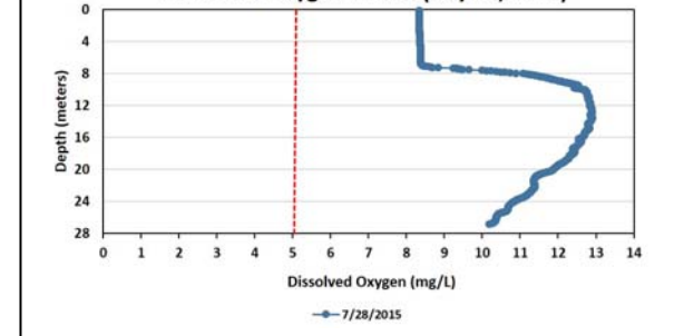
Figure 6. Merrymeeting Lake - Site 1 Broad Cove Dissolved Oxygen Profile (July 28, 2015)
