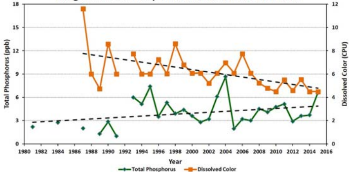
Figure 5. Merrymeeting Lake - Site 1 Broad Cove (1981-2015) Long-term Total Phosphorus and Dissolved Color Data
