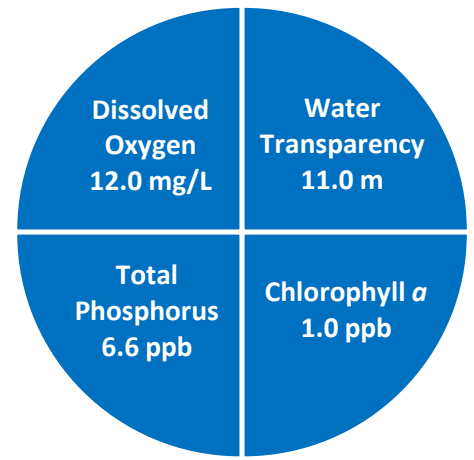
Figure 1. Merrymeeting Lake Water Quality (2015)
